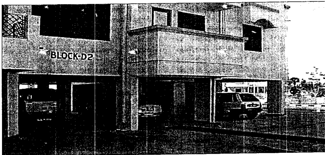
Figure 5: RC Frame Buildings with columns in open ground storey of 230mm width
